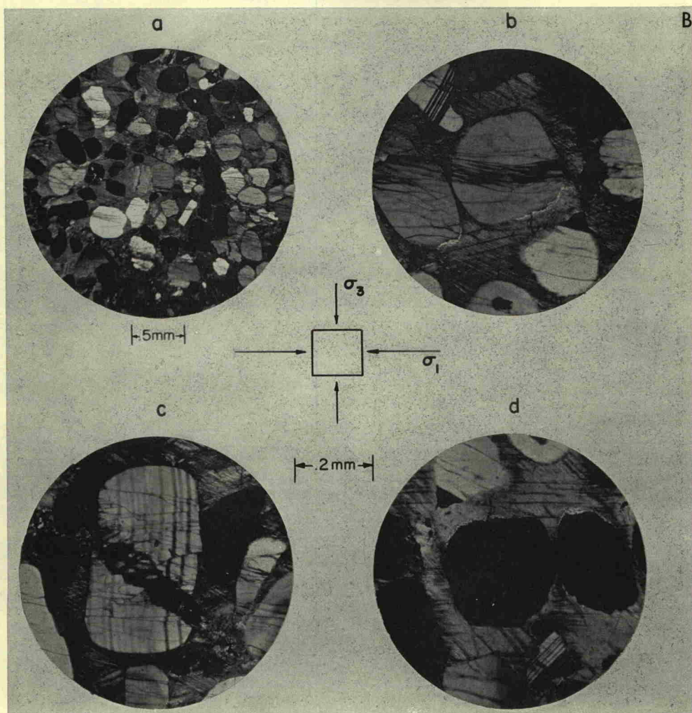
Sand crystals and photomicrographs of details of specimen 911
